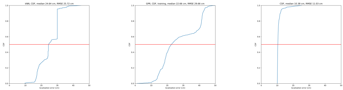
Fig. 7: CDF curves of localization error for the k NN, GPR and the proposed BCL coordinate estimation methods.
