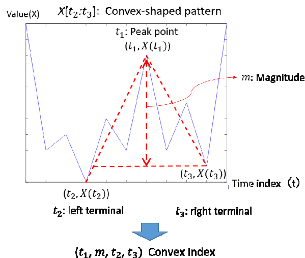
Figure 3: An example of a convex-shaped pattern and its convex index
