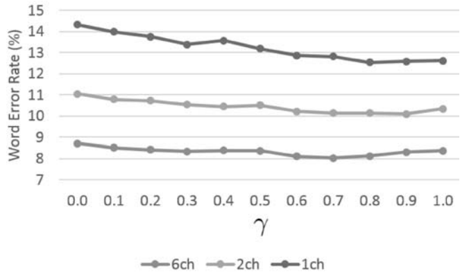
Fig. 4. Proposed student-teacher learning with enhanced speech for CHiME-4 development set (1, 2, and 6 channel tracks).
