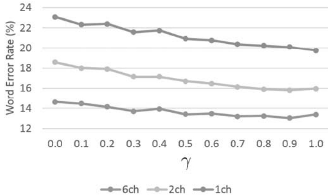
Fig. 5. Proposed student-teacher learning with enhanced speech for CHiME-4 evaluation set (1, 2, and 6 channel tracks).
