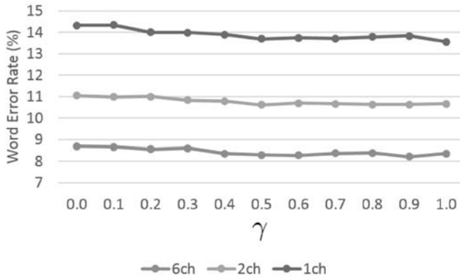
Fig. 2. Student-teacher learning with noisy speech for CHiME-4 development sets (1, 2, and 6 channel tracks).
