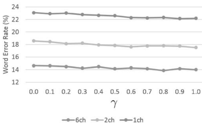
Fig. 3. Student-teacher learning with noisy speech for CHiME-4 evaluation set (1, 2, and 6 channel tracks).
