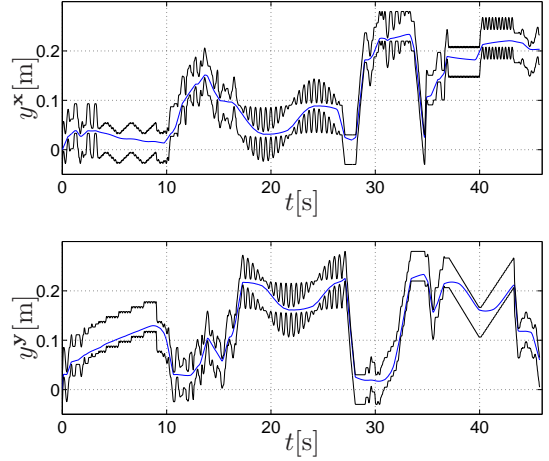
Fig. 3. Position of the slow stage x, y axes (blue) and constraints (black) due to the reference and fast stage range
