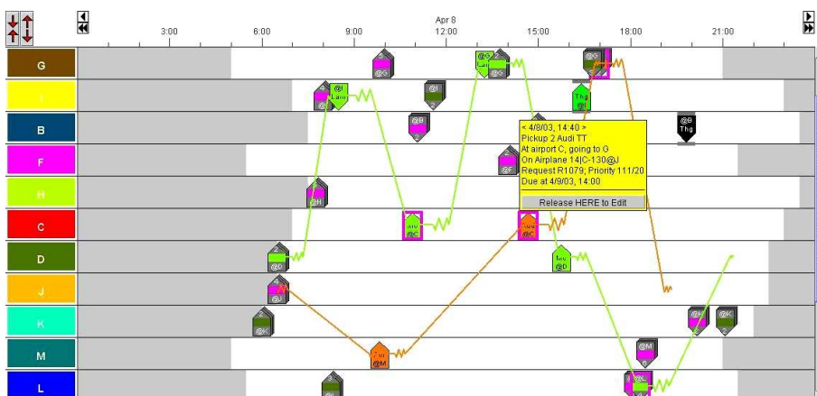
Figure 3. Detailed View (Zoom = 1-Days, Base Elements = Airports, Coloring Schemes = Airplanes, no Filters): flightroutes are shown for the marked operations; a tooltip for detailed information on a request
